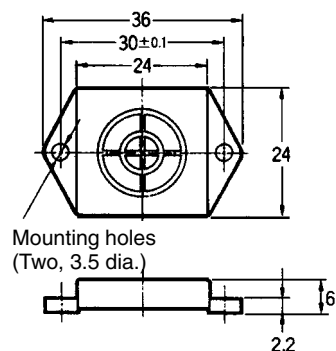
V600-D23P61
