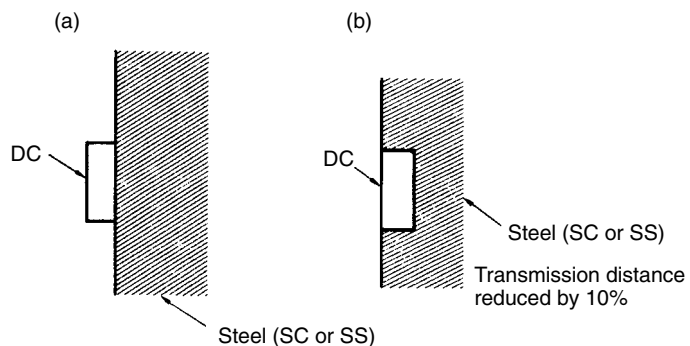
(a) Mounting to Metal Surface (b) Embedding in Metal
