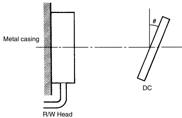
(1) Reduction in Transmission Distance for Misalignment in V600-D23P66SP
