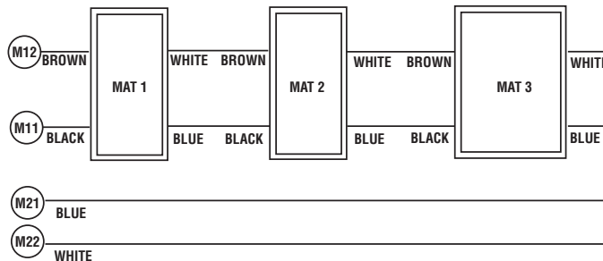
Figure 5-1 Hookup Drawing
