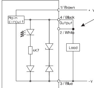
PNP NC Output
