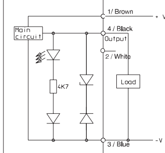
PNP NO Output
