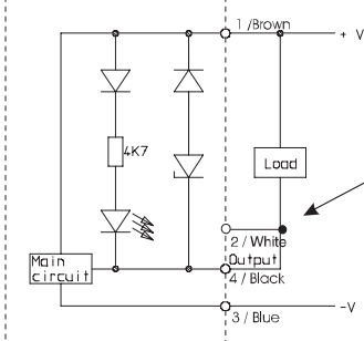
NPN NC Output
