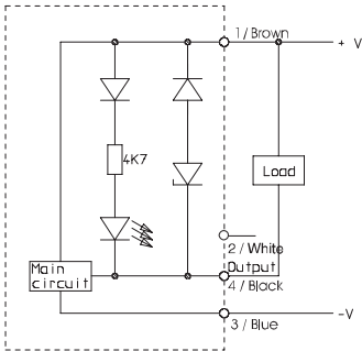
NPN NO Output
