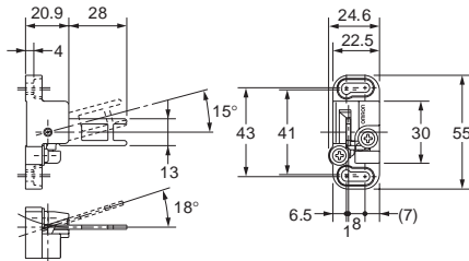
Adjustable Mounting (Horizontal/Vertical) D4DS-K5
