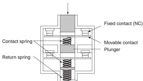
2NC Contact (Slow-action)
