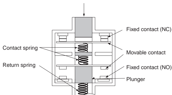
1NC/1NO Contact (Slow-action)
